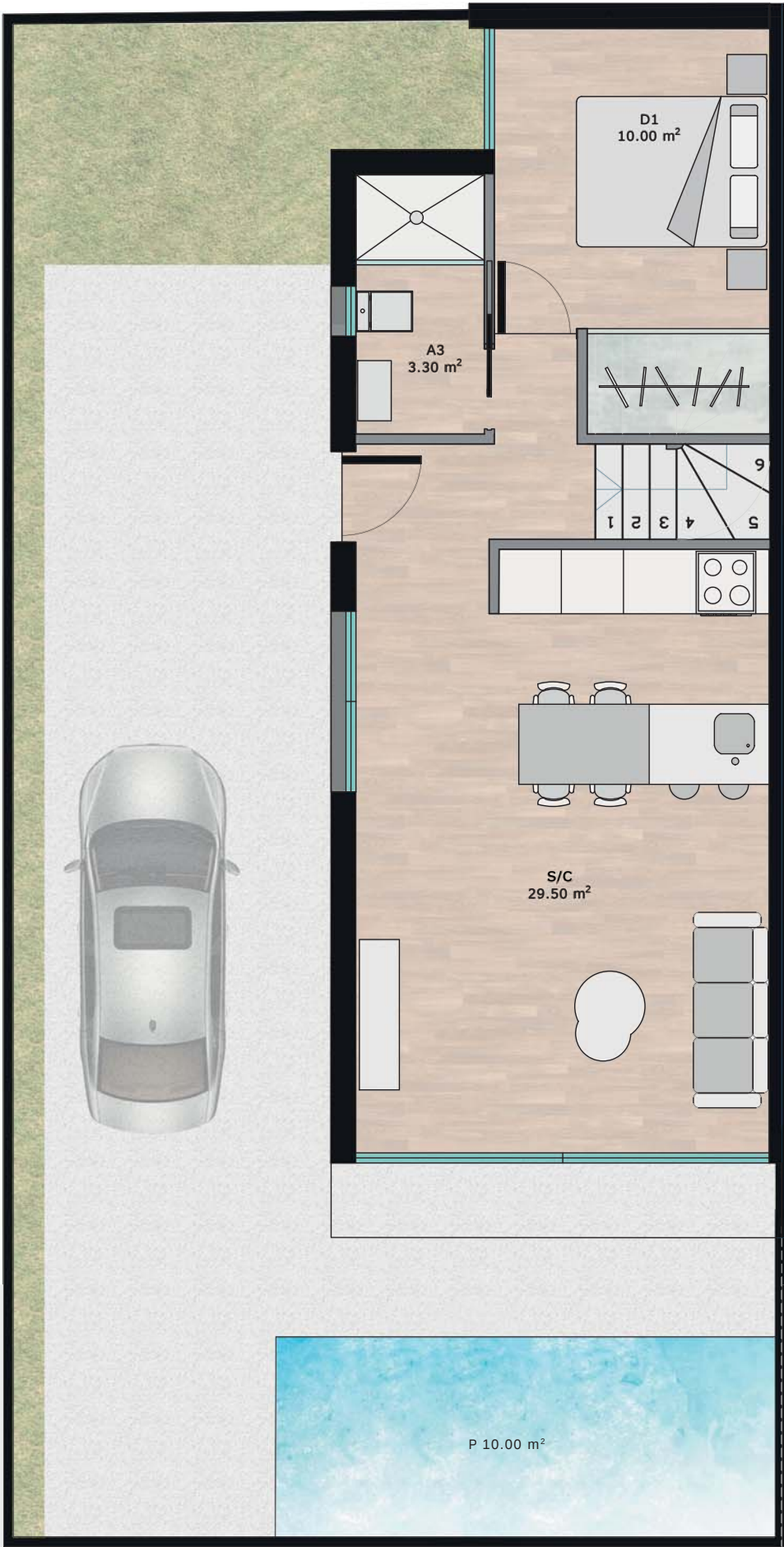
FIRST FLOOR
